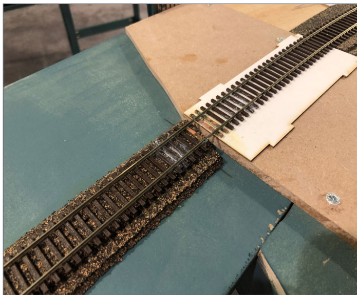
6. Closed position. Using PCB ties on both the gate and the layout to help keep the rails aligned at the gate.
