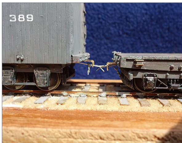
29. A trial version of the Alex Jackson coupling.
