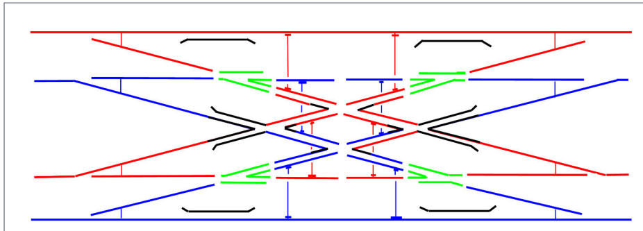
7. Walthers Code 83 Double Crossover Wiring Schematic-jumpers shown.
