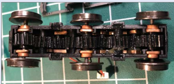
25. The newer Walther's Proto SD9 truck power pickup differs greatly from the older Proto 2000's. The problematic copper sideframes are gone.
