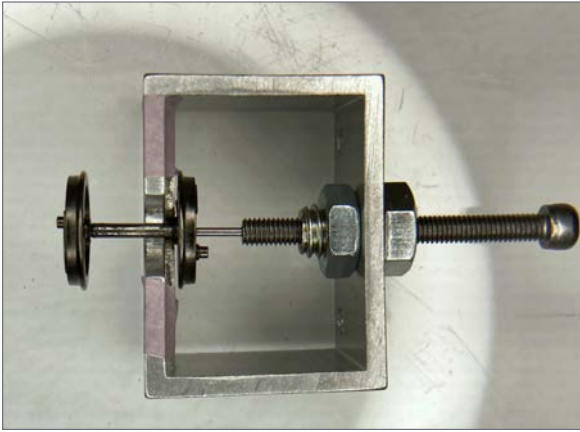
12. Removing the wheelset in The Puller.
