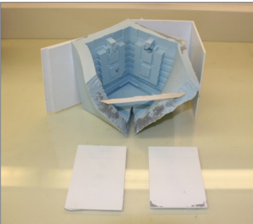
7. Mold for the four-sided towers split apart is needed to remove the master and copies.
